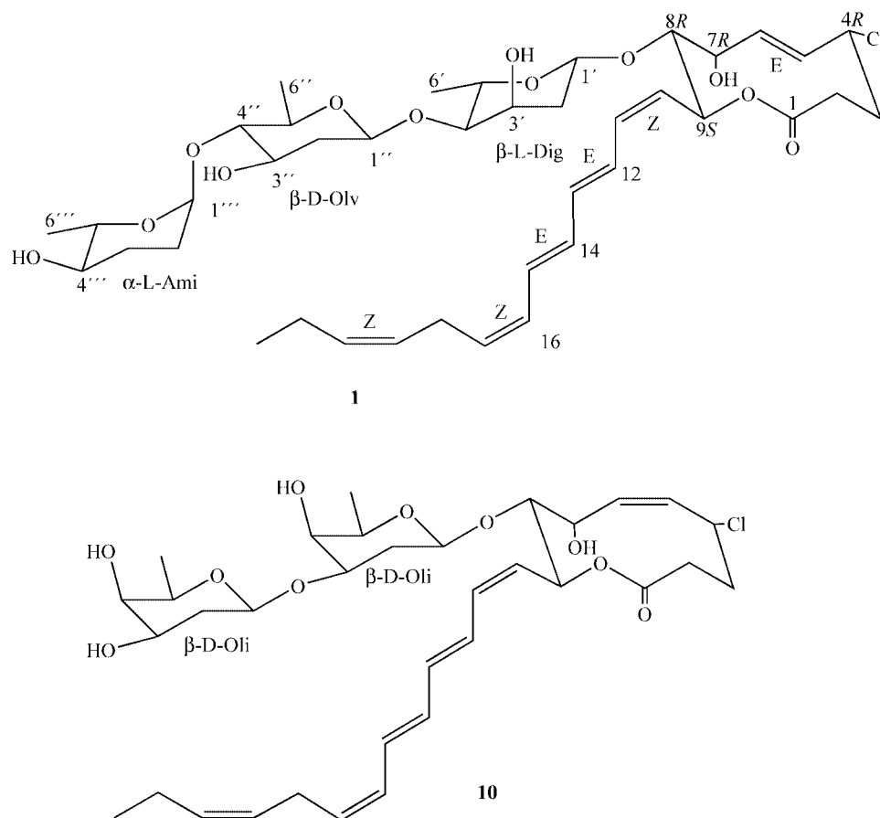
Figure 1. Structure of new glucosides (latrunculinosides A and B; 1 and 10 ) from Latrunculia corticata , a Red Sea sponge
