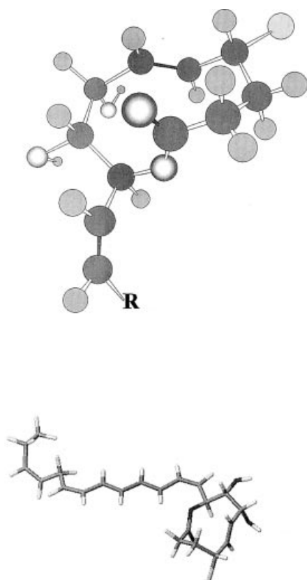
Figure 4. 3D-MM2 models (with and without side chain) of compound 1 are included
