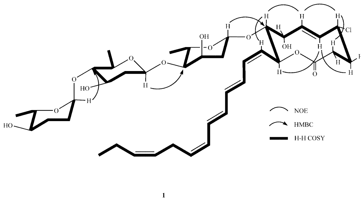
Figure 3. The NOE, HMBC, and H-H COSY correlations of latrunculinoside A ( 1 )
