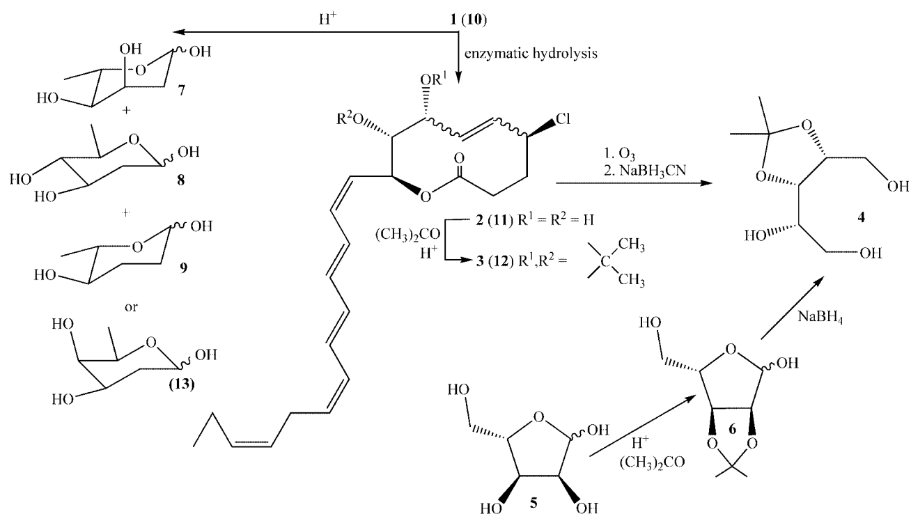
Figure 2. Reaction schemes for degradation compounds from glycoside 1 ( 10 ) and synthesis of standard 2,3- O -isopropylidene-L-ribitol ( 4 )
